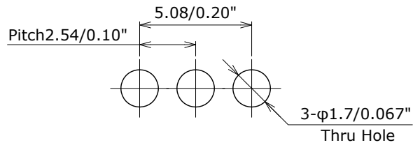
PC Board Layout (Top View)
