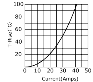
T4P-L214-ST-BK-P T-Rise Current Chart Between Drain and Source(Reference)
