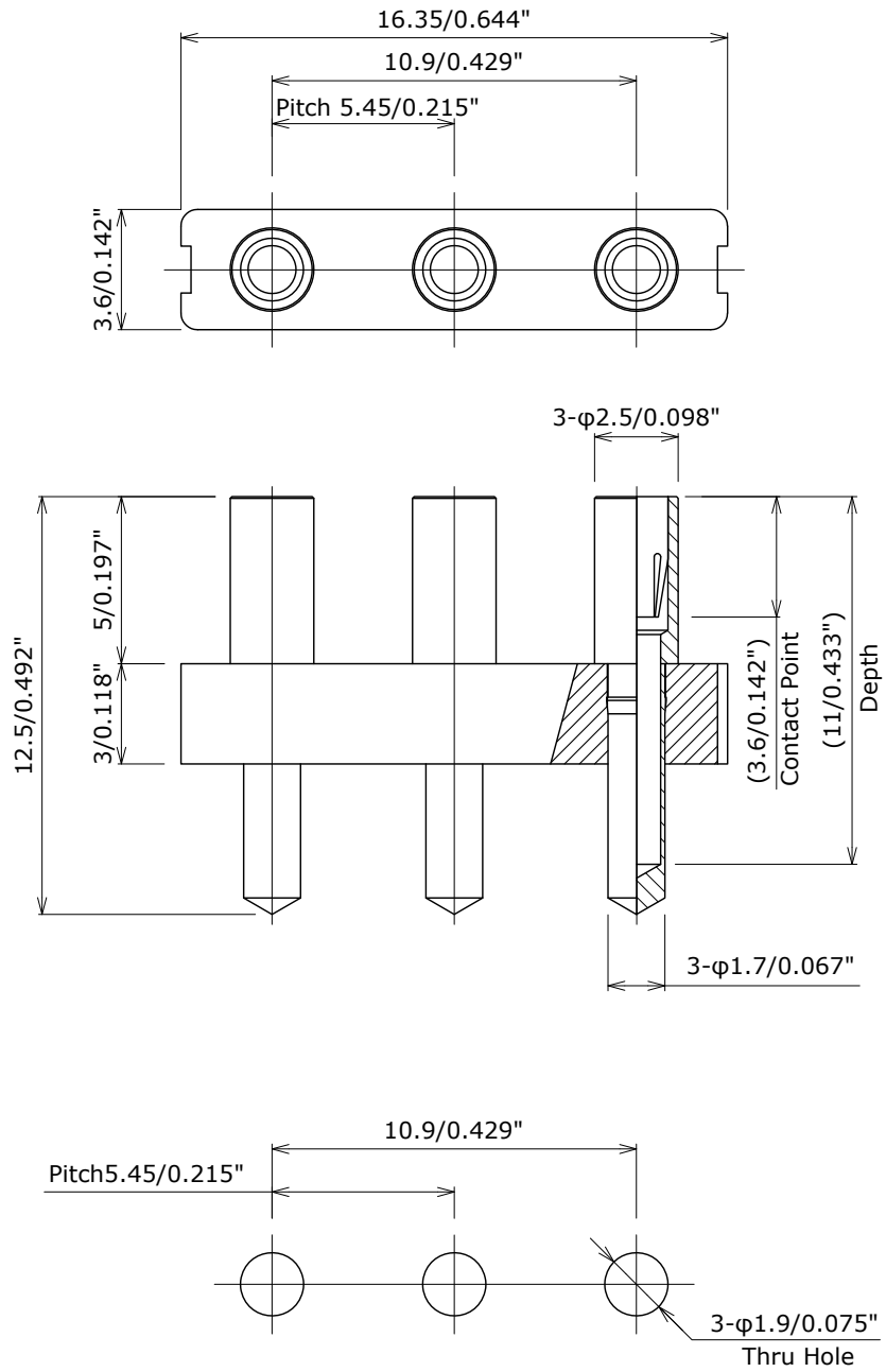
PC Board Layout (Top View)
